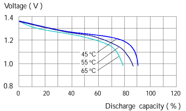
Discharge Curves ( 1400 mA )
