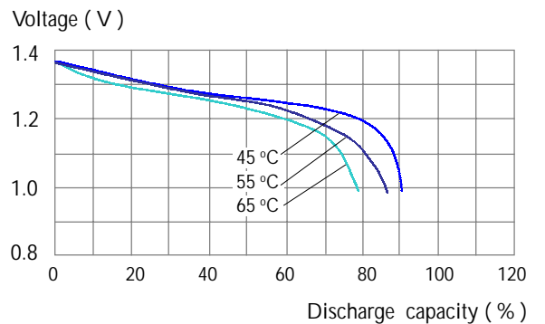
Discharge Curves ( 1000 mA )
