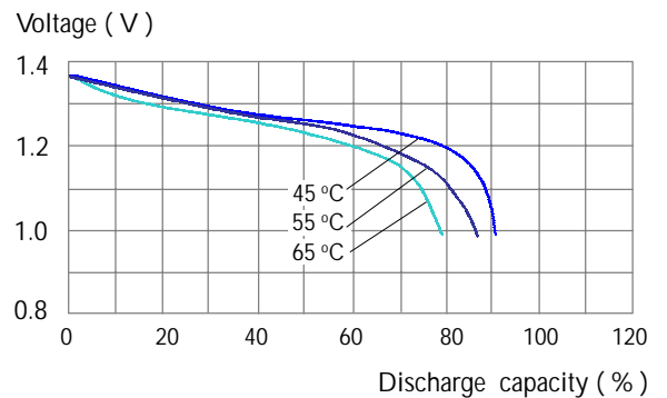
Discharge Curves ( 140 mA )
