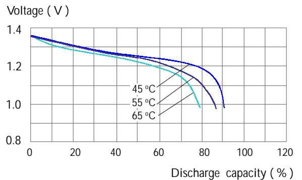
Discharge Curves ( 120 mA )
